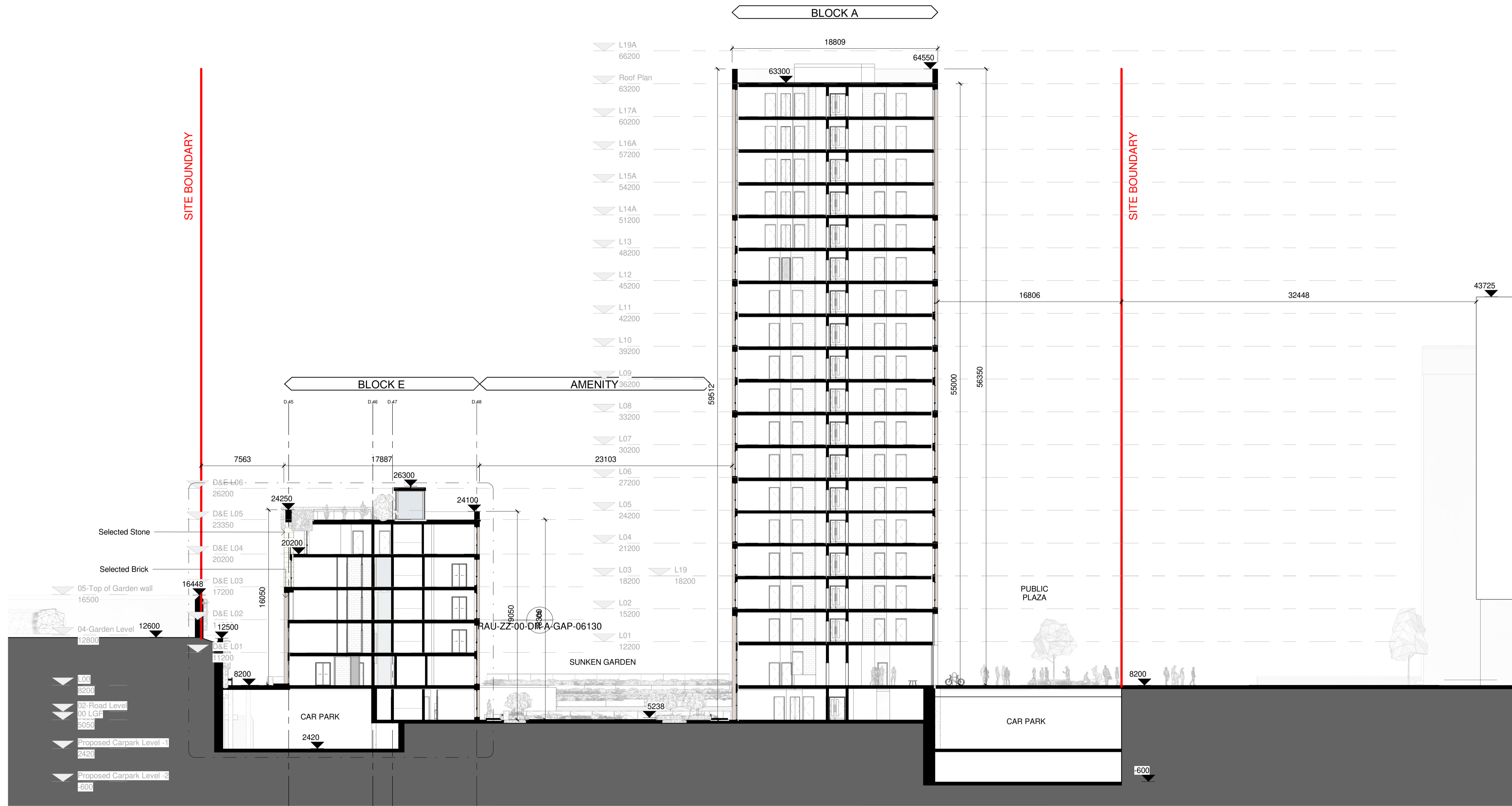
Proposed Section 02 1:200
